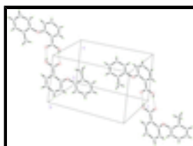
Fig. 2. Packing diagram for (I). O—H···O hydrogen bonds are shown by dashed lines.
